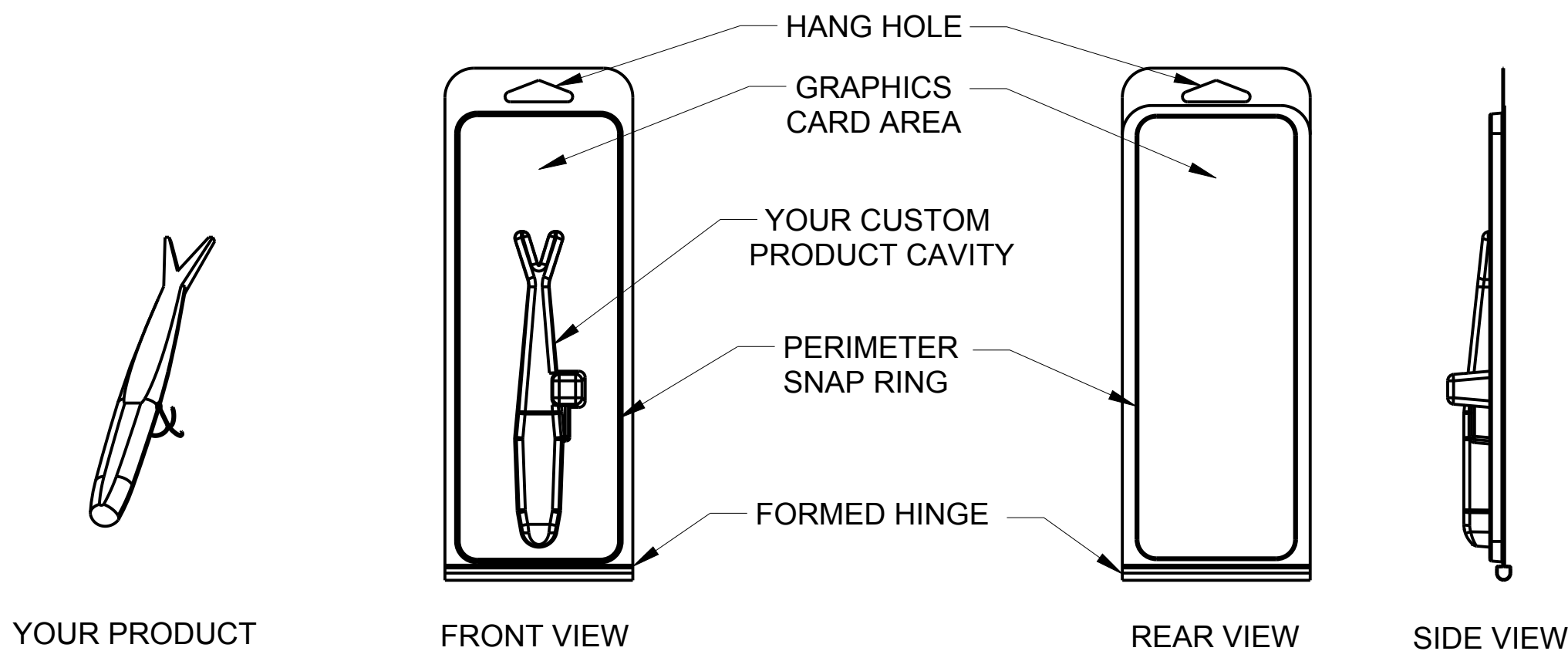
SEMI-CUSTOM CLAMSHELL THAT CUSTOM FITS YOUR PRODUCT
